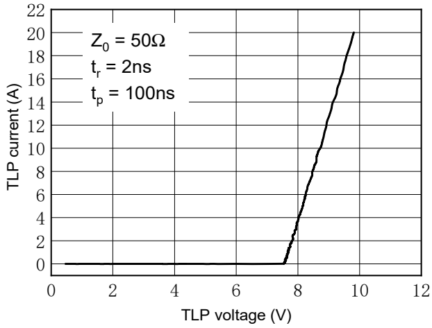
Fig.9 TLP Measurement
